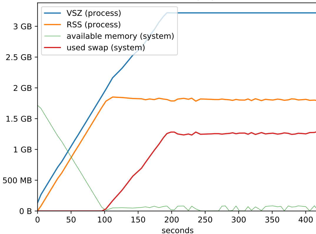
fibn test with comp-speed 0
