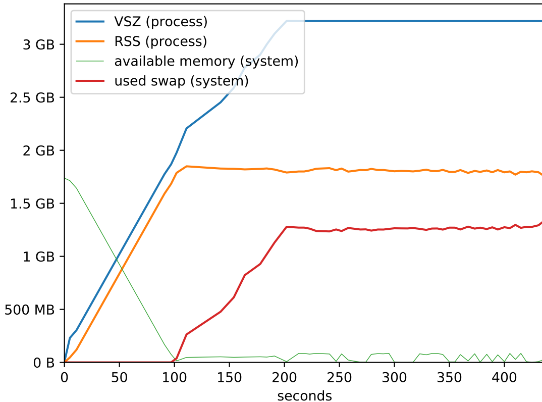
fibn test with comp-speed 3
