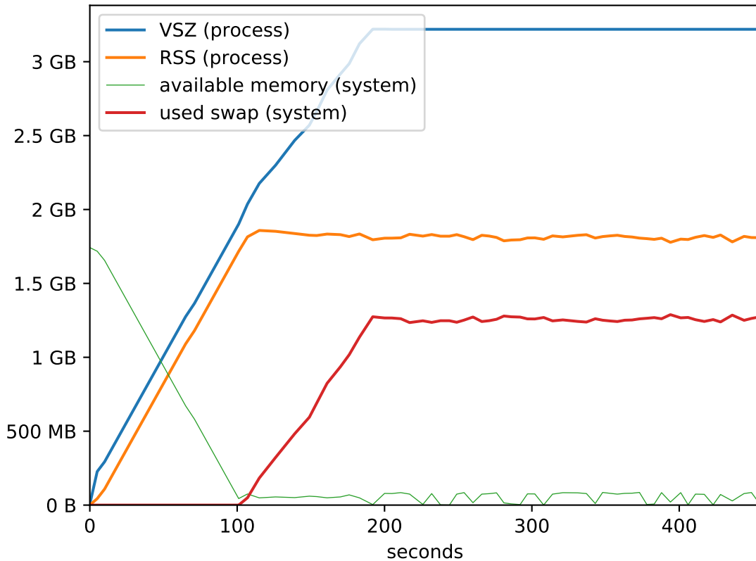
fibn test with comp-speed 2
