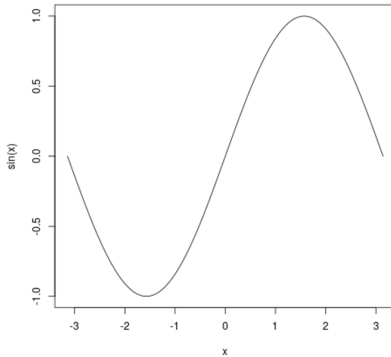
Figure 1: Figure generated by R
