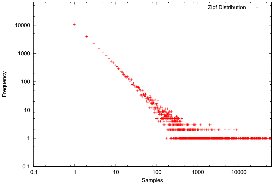
Zipf distribution
